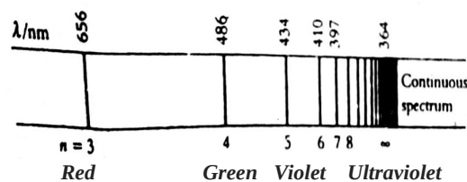
The Balmer series of hydrogen
