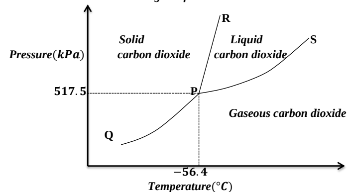
Phase diagram for carbon dioxide
