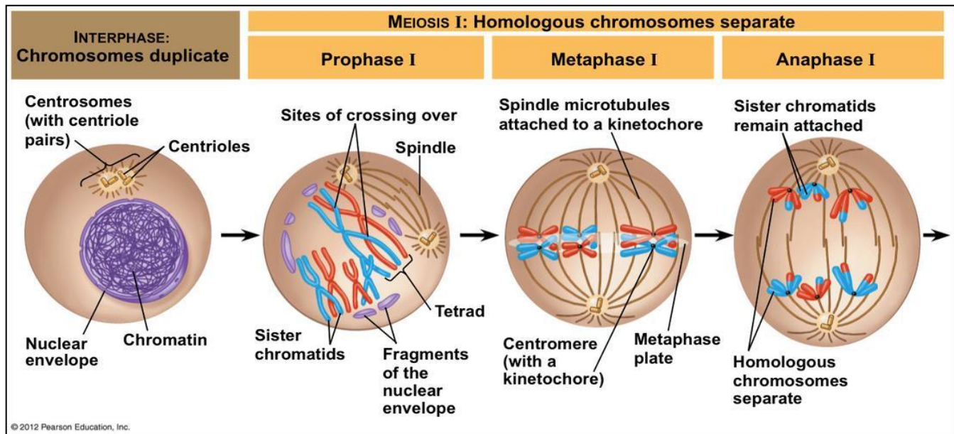
Figure 1: Meiosis I
