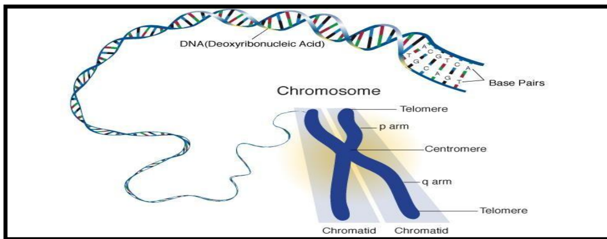
Figure 3: Chromosomes structure
