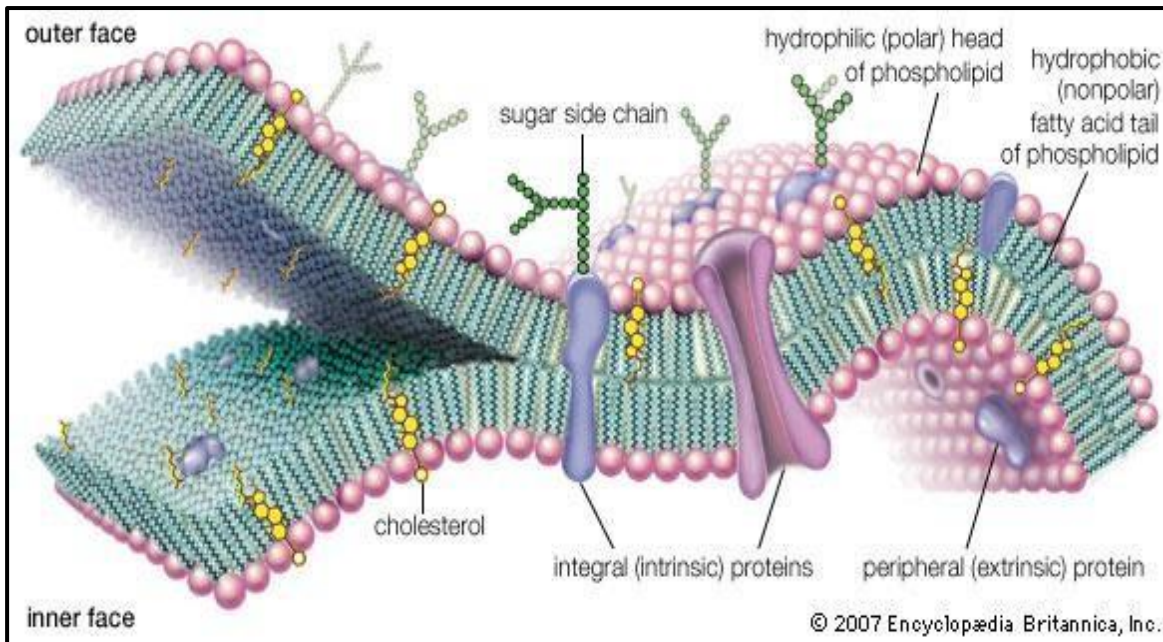
Figure 1: Cell membrane
