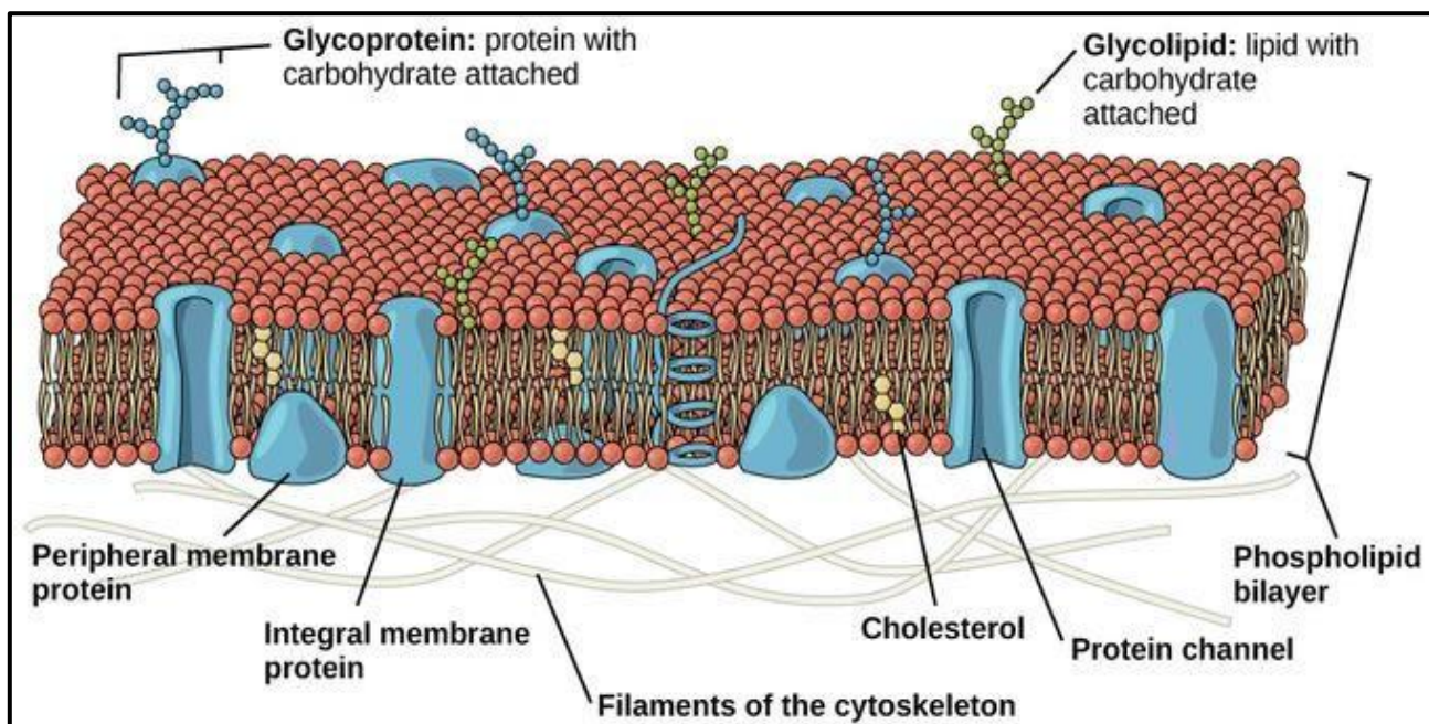
Figure1: Eukaryotic Plasma Membrane: The eukaryotic plasma membrane is a phospholipid bilayer with proteins and cholesterol embedded in it.
