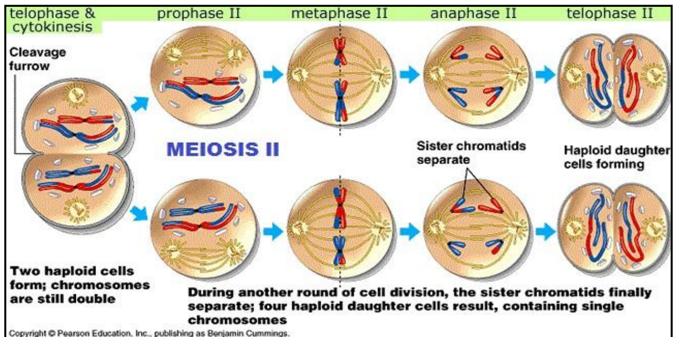
Figure 2: Meiosis II
