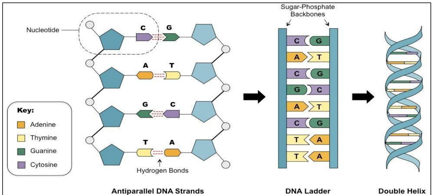
Figure 2: DNA structure
