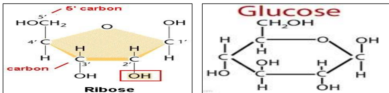
Figure 1: Ribose and Glucose molecule
