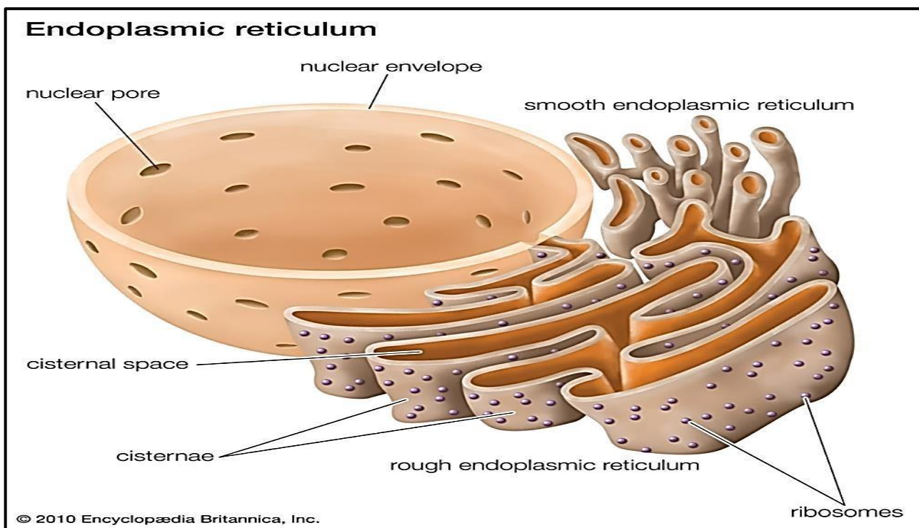
Figure 4: Endoplasmic reticulum
