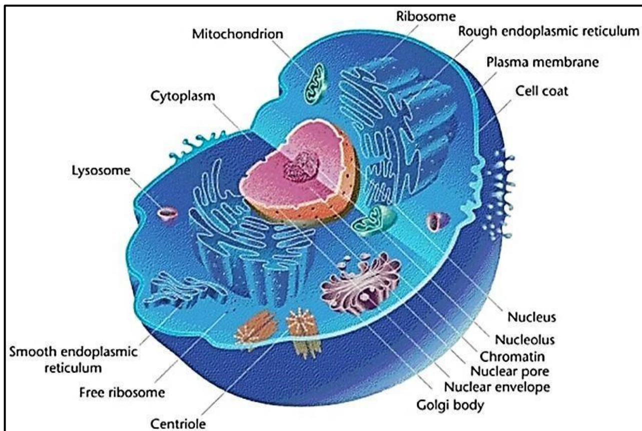
Figure 2: The animal cell.
