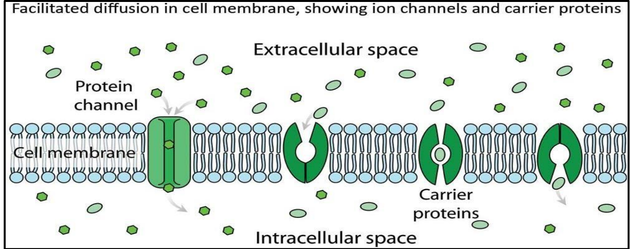
Figure 3: Facilitated Transport
