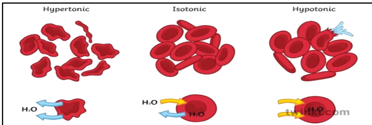
Figure 4 : Osmosis
