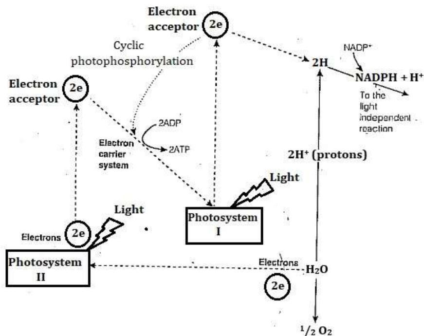
Figure 9: The Z-Scheme
