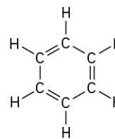
Benzene ( \mu = 0 )
