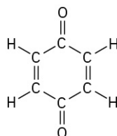
Benzoquinone
