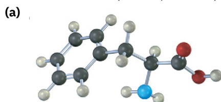
Phenylalanine
