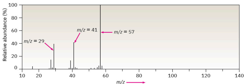
FIGURE 12.5 Mass spectrum of 2,2-dimethylpropane ( \text{C}_5\text{H}_{12} ; MW = 72). No molecular ion is observed when electron-impact ionization is used. What do you think is the formula and structure of the \text{M}^+ peak at m/z = 57 ?
