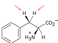
Phenylalanine
