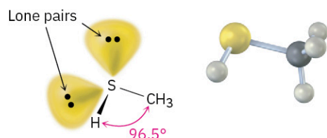
Methanethiol
