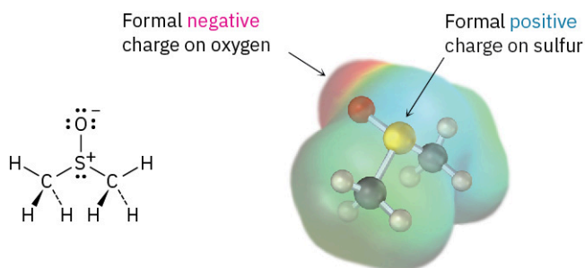
Dimethyl sulfoxide
