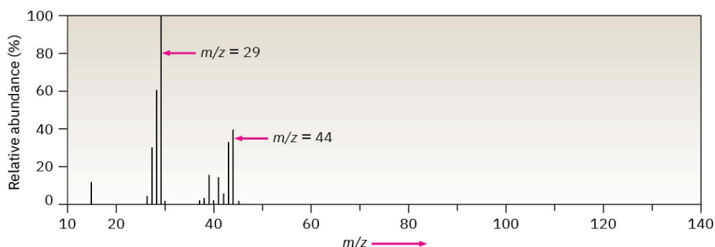
FIGURE 12.4 Mass spectrum of propane ( \text{C}_3\text{H}_8 ; MW = 44).
