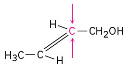
Crotyl alcohol
