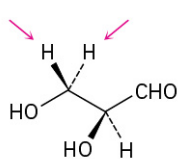
(S)-Glyceraldehyde
