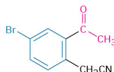
9. (2-Acetyl-4-bromophenyl)acetonitrile
