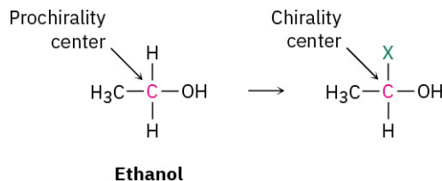
Ethanol
