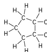
1,2-Dichlorocyclopentane
