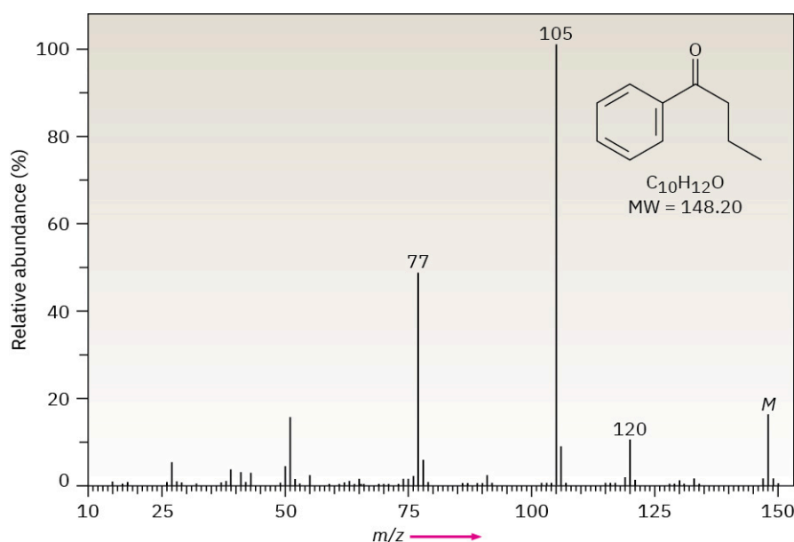
FIGURE 12.14 Mass spectrum of butyrophenone.
