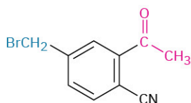
8. 2-Acetyl-(4-bromomethyl)benzonitrile
