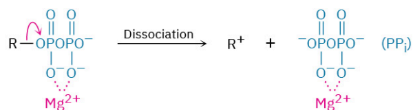
An organodiphosphate
