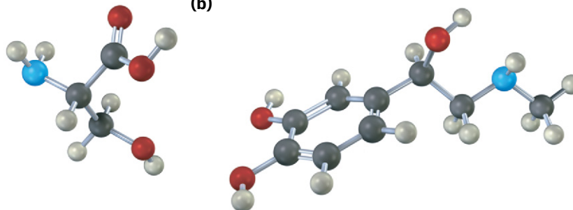
Serine
