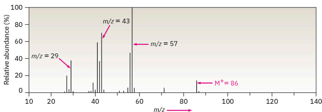
FIGURE 12.6 Mass spectrum of hexane ( \text{C}_6\text{H}_{14} ; \text{MW} = 86 ). The base peak is at m/z = 57 , and numerous other ions are present.
