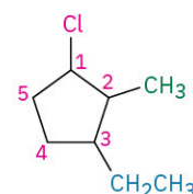
1-Chloro-3-ethyl-2-methyl- cyclopentane
