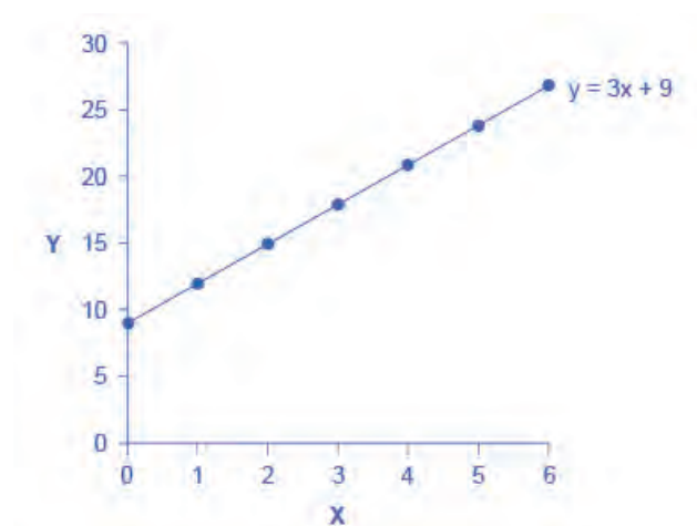
Figure A1 Slope and the Algebra of Straight Lines This line graph has x on the horizontal axis and y on the vertical axis. The y -intercept—that is, the point where the line intersects the y -axis—is 9. The slope of the line is 3; that is, there is a rise of 3 on the vertical axis for every increase of 1 on the horizontal axis. The slope is the same all along a straight line.
