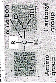
Structure of amino acids
