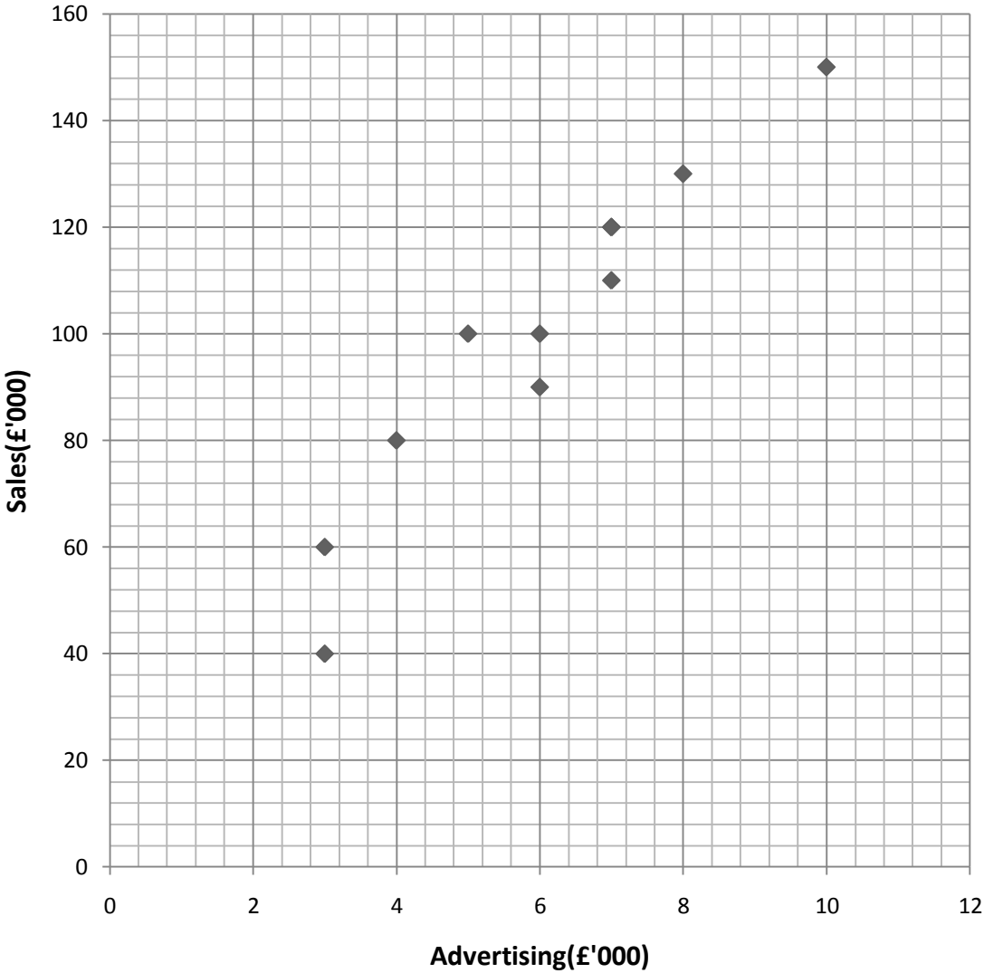
Scatter diagram
