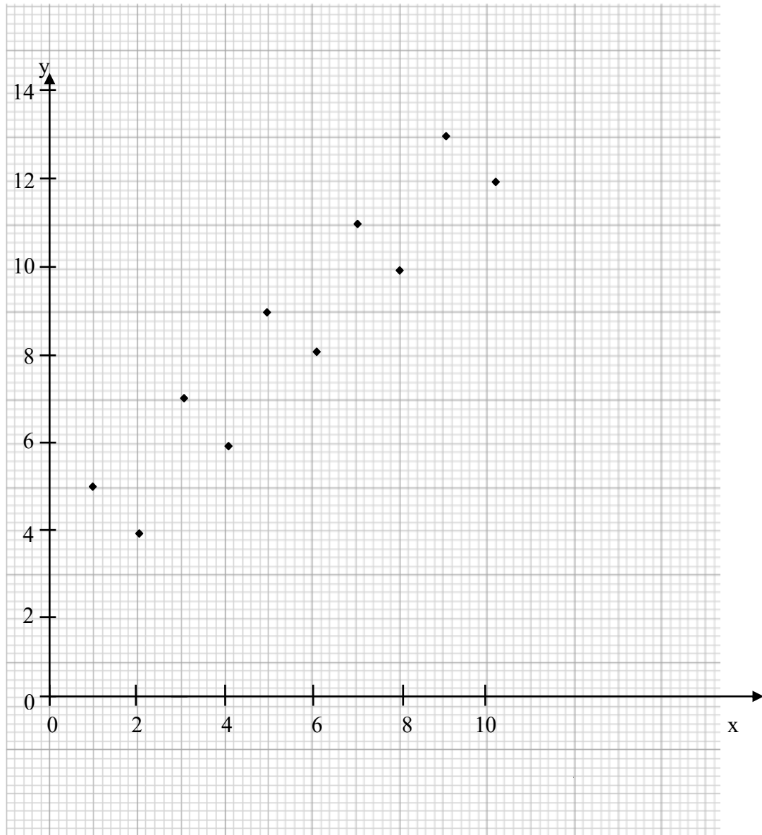
Scatter Graph
