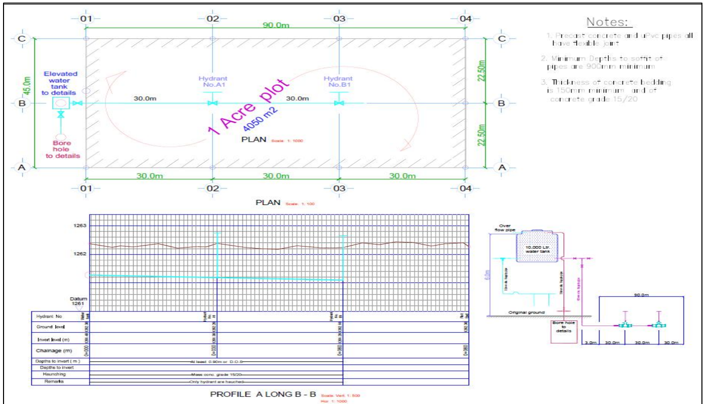
Figure 1: 1-Acre Fodder Multiplication Plot and water infrastructure Layout | DRG No. JN-001 | See attached detailed drawing to scale.
