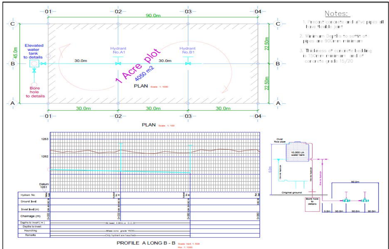
Figure 1: 1-Acre Fodder Multiplication Plot and water infrastructure Layout | DRG No. JN-001 | See attached detailed drawing to scale.
