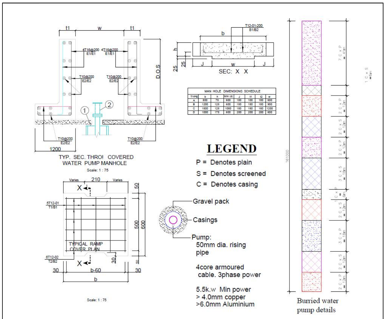
Figure 2: Borehole and Borehole Chamber Design| See attached drawing done to scale
