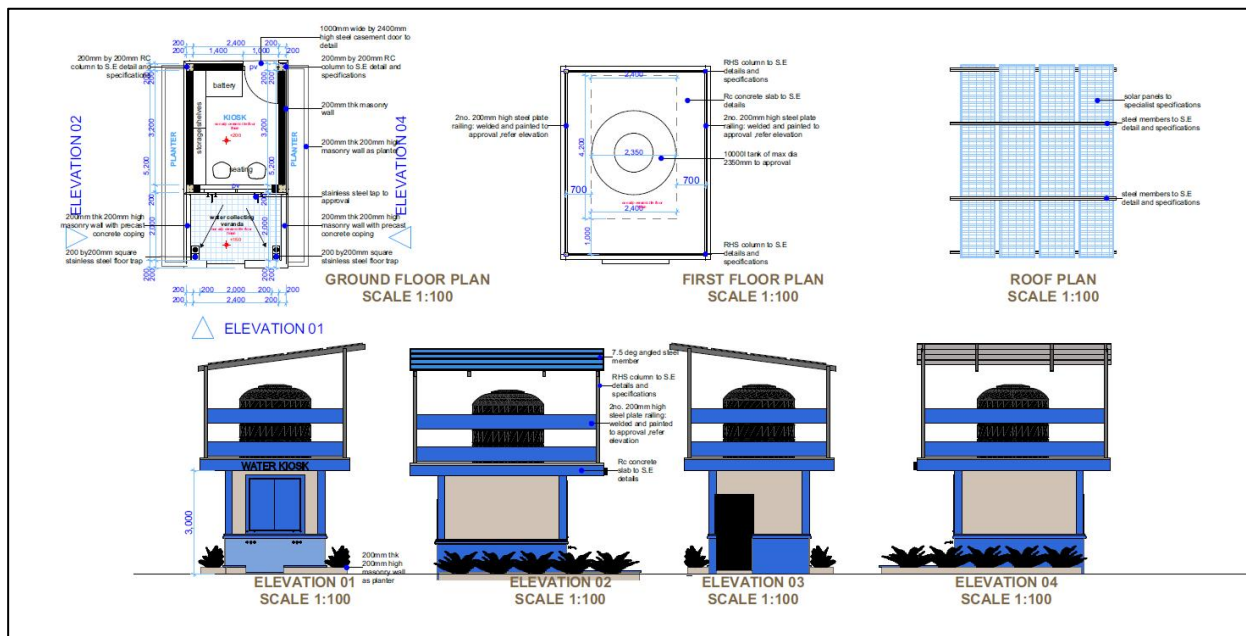
Figure 2: Elevations of the Water Kiosk showing the masonry structure (concrete frame, stone walling, non-slip ceramic floor tiles), 10,000-litre HDPE plastic tank mounted on the kiosk roof at \approx 3.5\text{m} above NGL, solar PV array of 10 \times \text{Dayliff } 325\text{W} panels on elevated mounting rack, 1\frac{1}{2} " UPVC rising main from borehole, 3.6 kW solar pumping inverter, and community tap outlets. (See attached drawings)
