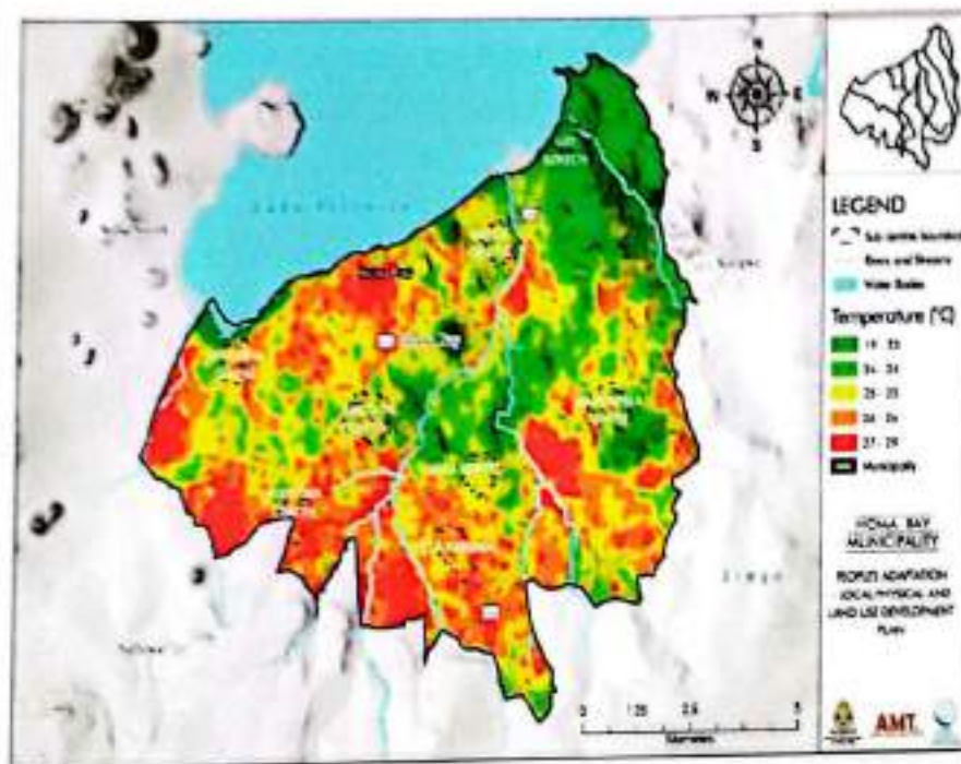
Figure 6: Surface Temperature prone areas.
